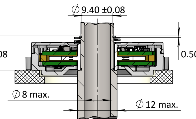
Midshaft with hollow shaft - example
