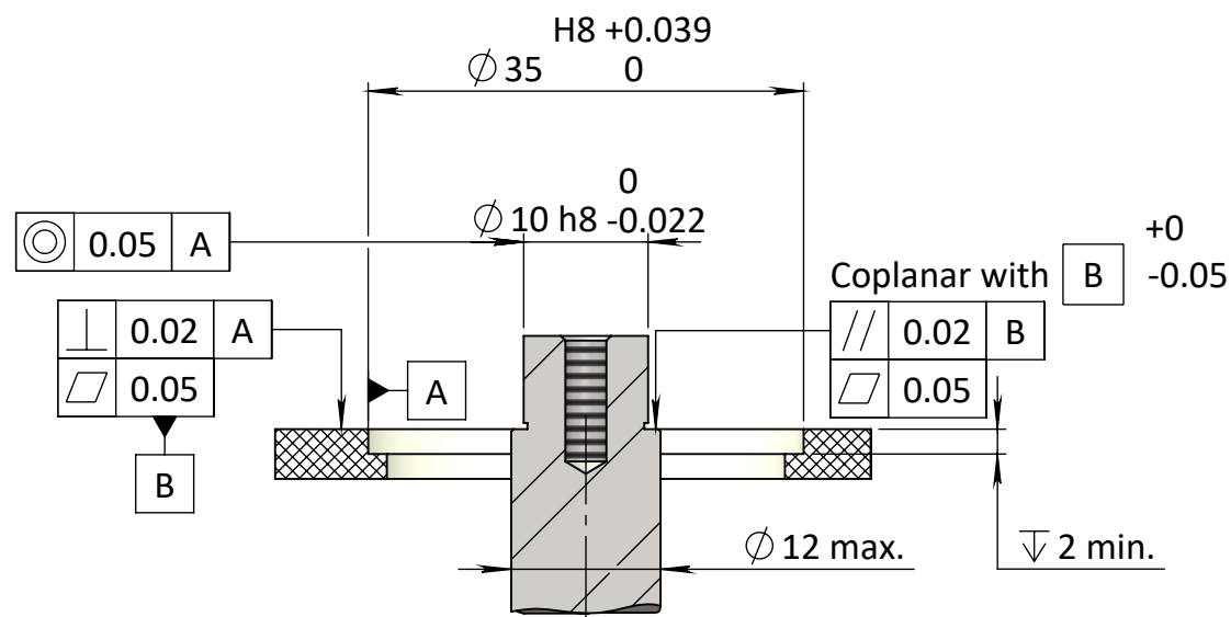
Typical mounting requirements
