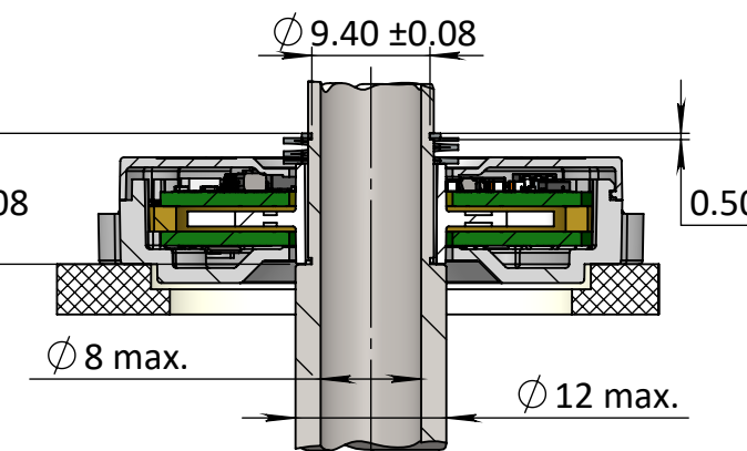
Midshaft with hollow shaft - example
