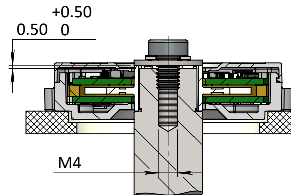
End-shaft with shoulder mounting - example
