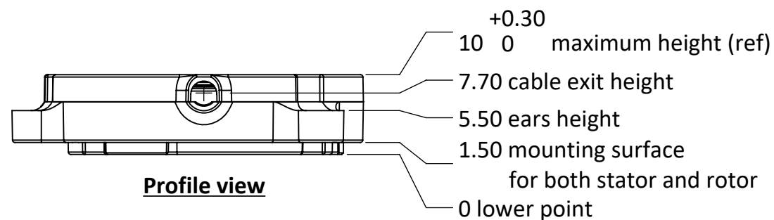
Typical mounting requirements
