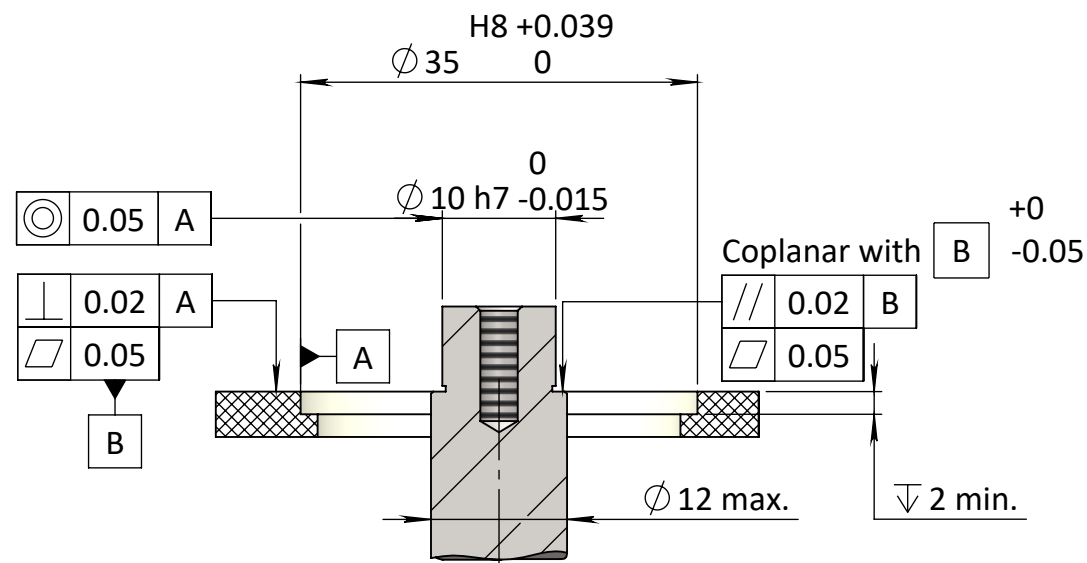
Typical mounting requirements
